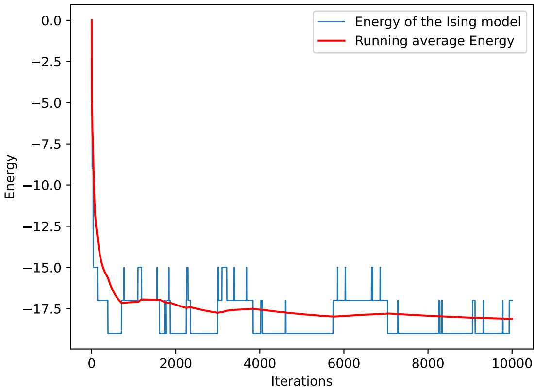
Evolution of a stochastic simulation of the 1D Ising model, at \beta = 2 J = 1 h = 0
